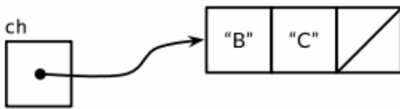
Figure 8.4. A partially full buffered channel.
