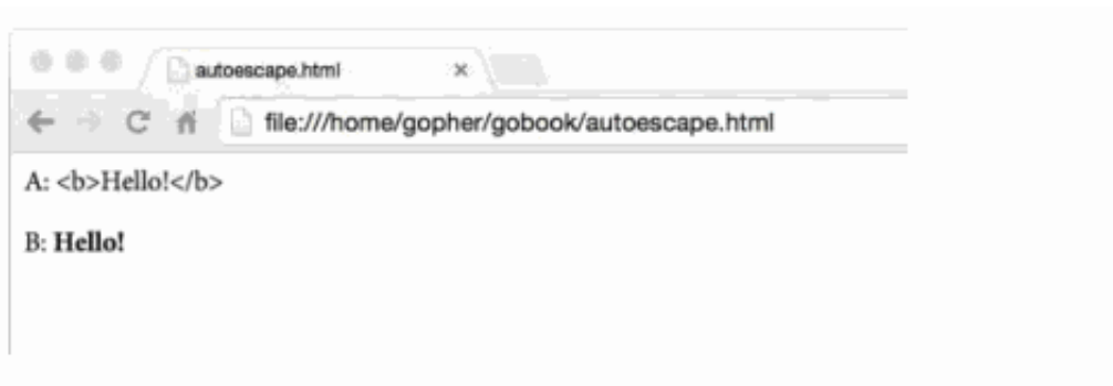
Figure 4.6. String values are HTML-escaped but template.HTML values are not.
