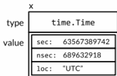
Figure 7.4. An interface value holding a time.Time struct.
